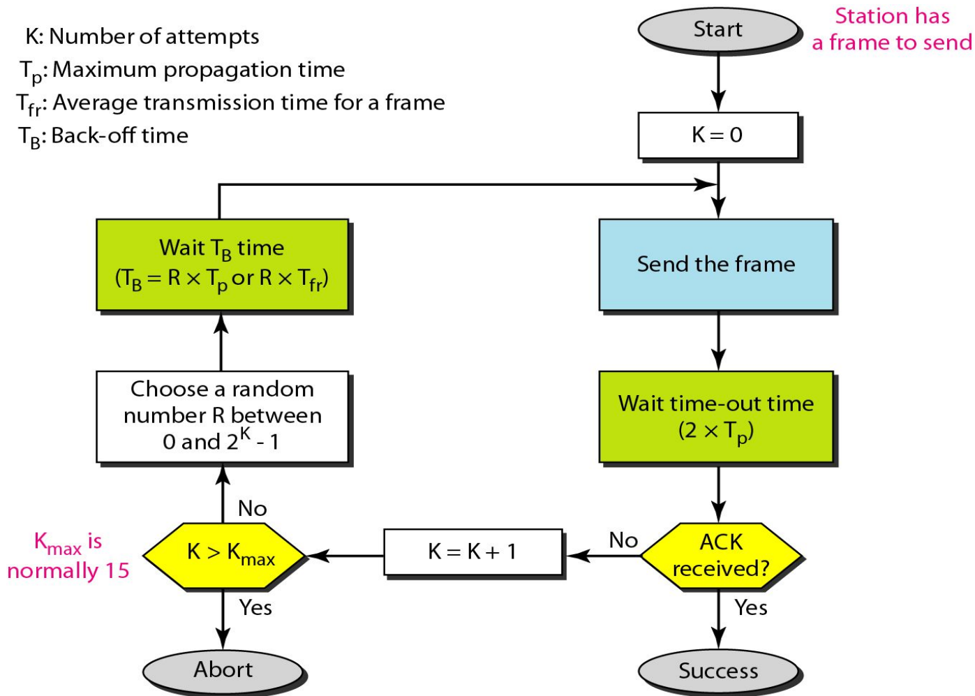
Figure 12.4 Procedure for pure ALOHA protocol
